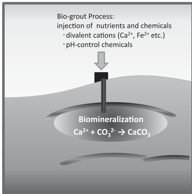
Fig. 3. Schematic representation of microbial enhanced CO 2 mineralization in the CCS site. Extensive security system of CCS is due to microbial induced carbonate precipitation (MICP).
