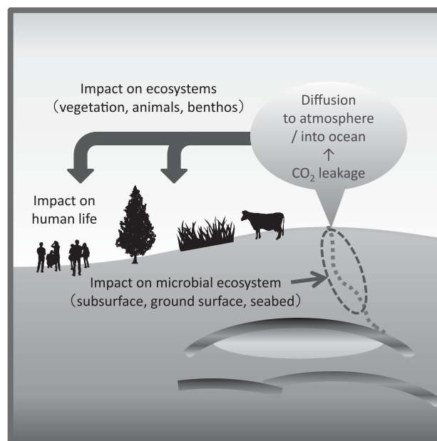
Fig. 1. Schematic representation of the environmental impacts due to CO 2 leakage
